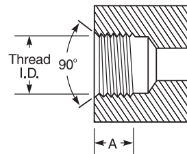
Female
