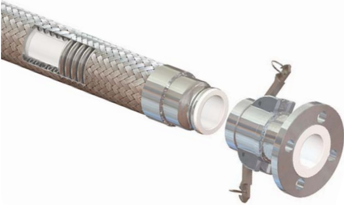
| Thorburn's 58TT PTFE metal hose assemblies | (PTFE "E" style male camlock hose ends can be attached to various PTFE lined adapters)
