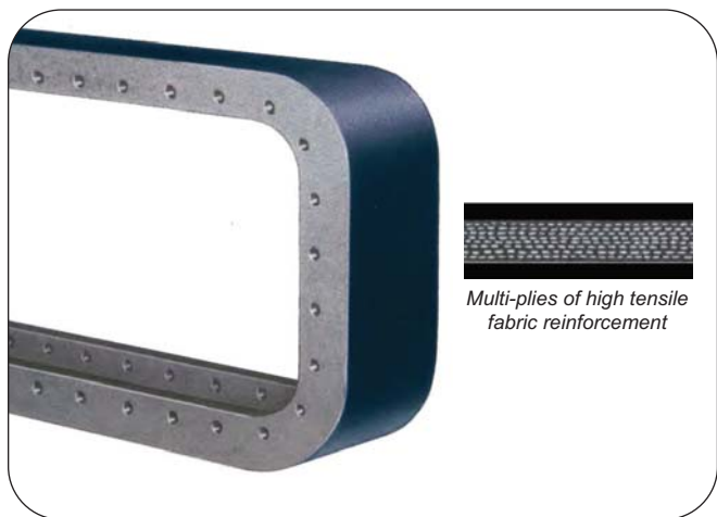
Thorburn's rubber "U-type" expansion joint with internal flange design
