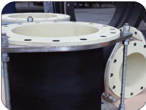
Thorburn Model 60RPC flanged pump connector with control rod assembly Type "CR"
