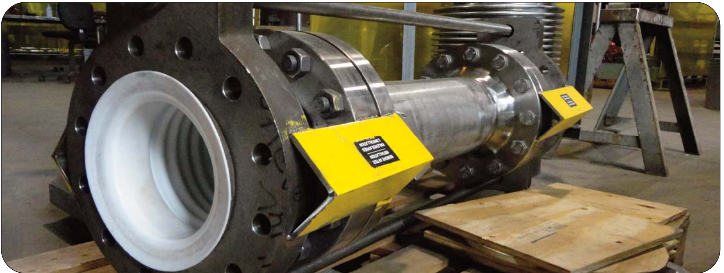
Thorburn's Hot-Flex high pressure PTFE lined expansion joint system with tangent pipe
