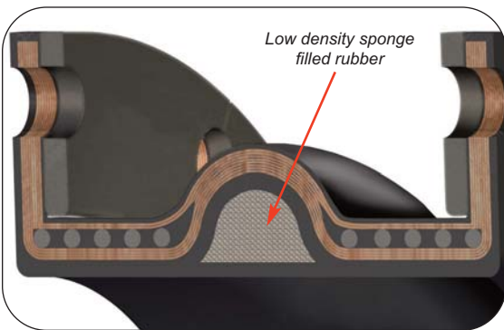
Thorburn's 42HPW high pressure expansion joint with a low density rubber filled arch is designed for smooth unrestricted flow and allows for 50% of open arch movement.
