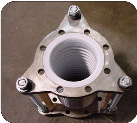
Thorburn's Hot-Flex with isostatically molded unpigmented PTFE convolutions
