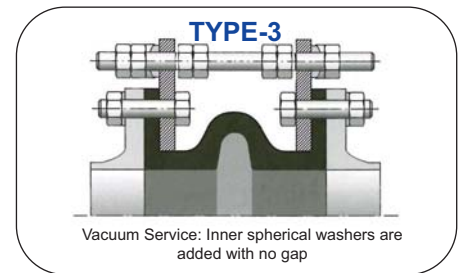
Vacuum Service: Inner spherical washers are added with no gap • Lateral movement • integral retaining ring & lug plate • Control rods with spherical washers & internal compression limiting nuts
