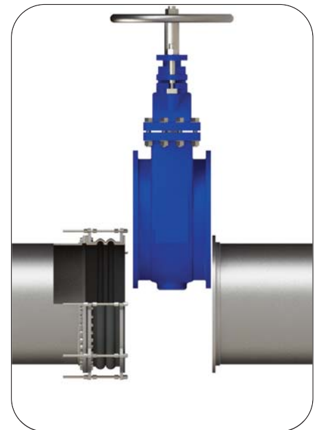
After Thorburn's dismantling joint has provided adequate space, the valve can easily be removed from the piping system
