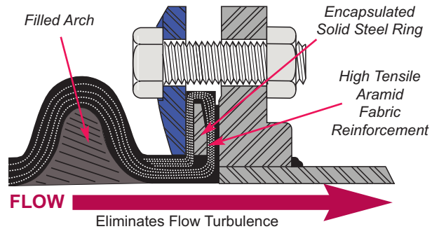
Interlocking Swivel Flanges
