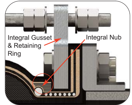
Thorburn Series 62HP-DJ for low to medium pressure applications
