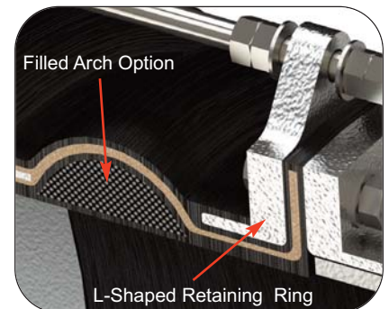
Thorburn Series 62HPWXX-DJ for high pressure applications
