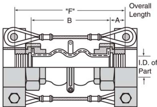
Thorburn's Model 102 standard union connector comes with control cables for added protection and to prevent over-extending leakage during start-up
