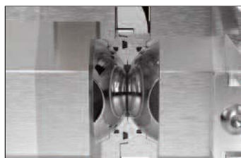
Ball Valve "Zero Gap" System
