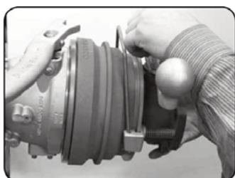
Connecting API coupling - a coupler (hose unit) with an adaptor (tank unit).
